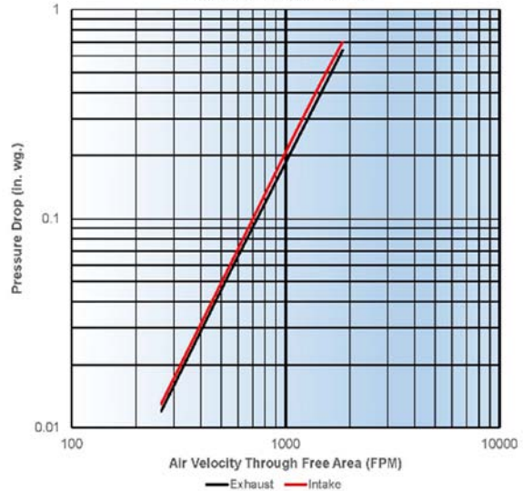
PRESSURE DROP 2210 / 2215 FIGURE 5.5 TEST SIZE 48" X 48"
